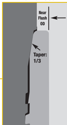
External Seal
