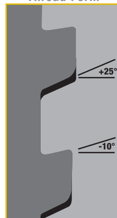
Thread Form
